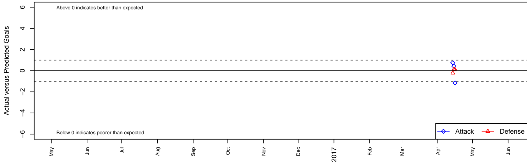
Calgary Northside Hurricanes B99 Dots are actual minus expected GF (blue circles) and GA (red triangles). Blue line is smoothed change in attack strength. Red is smoothed change in defense strength.
